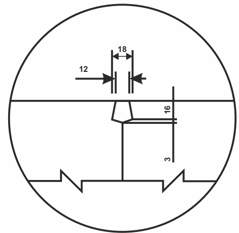
Typical Groove for Joint
